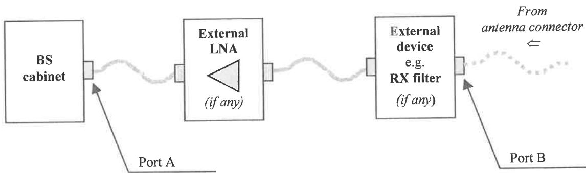
Gambar 2. Interface penerima BS type 1-C.
