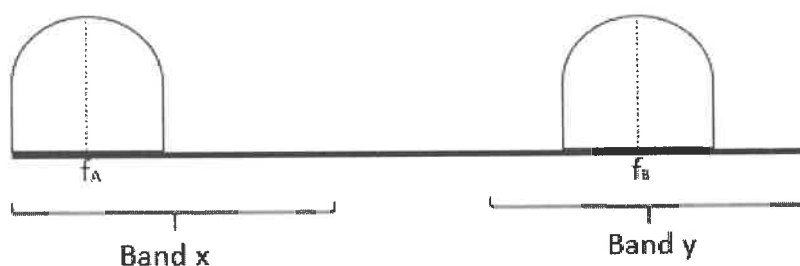
Gambar 3. Interband
