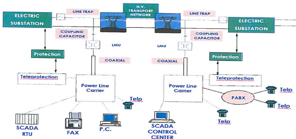
Gambar 1. Contoh konfigurasi sistem Single Sideband Power Line Carrier
